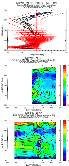
Figure 3. Temperature Differences of MIPAS/HALOE
