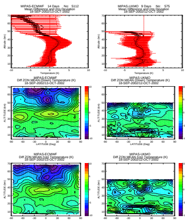
Figure 1. Temperature Differences of MIPAS/ECMWF and MIPAS/UKMO
