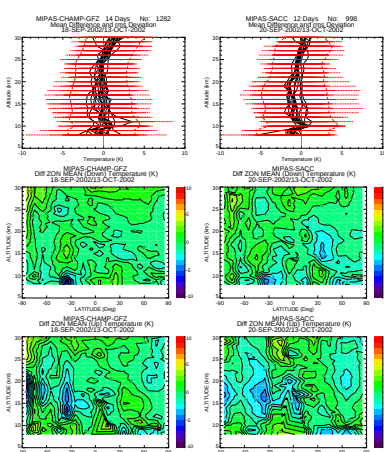
Figure 2. Temperature Differences of MIPAS/CHAMP and MIPAS/SAC-C
